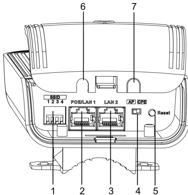
Figure 1-1 Device Interface/Button
