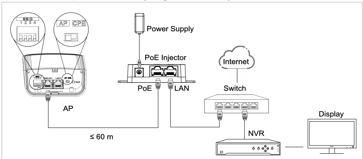
Figure 2-3 AP Connection
