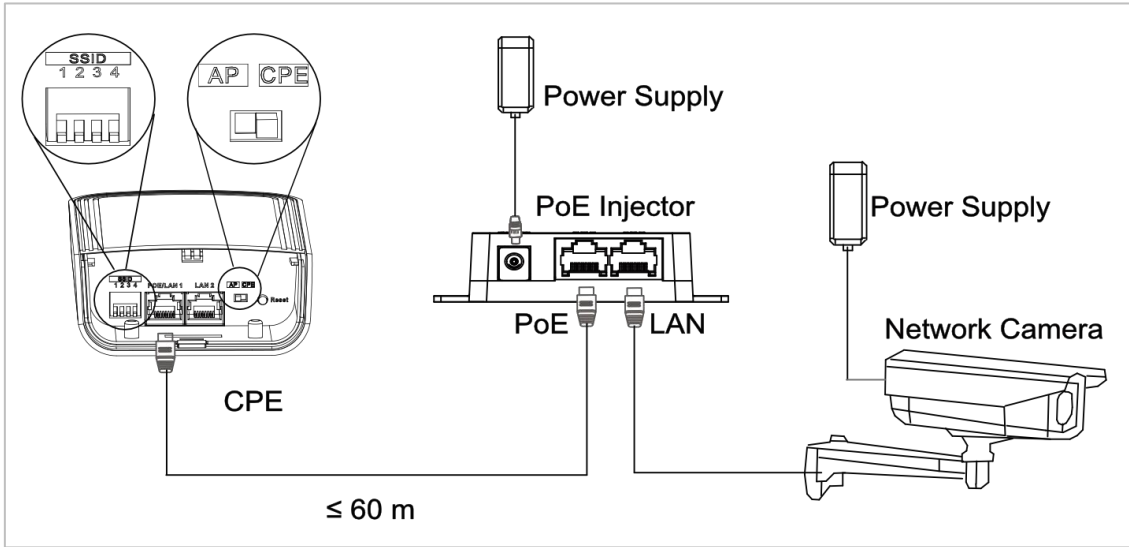
Figure 2-4 CPE Connection
